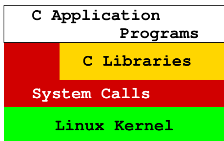
FIGURE 9.2: Library and System Calls
