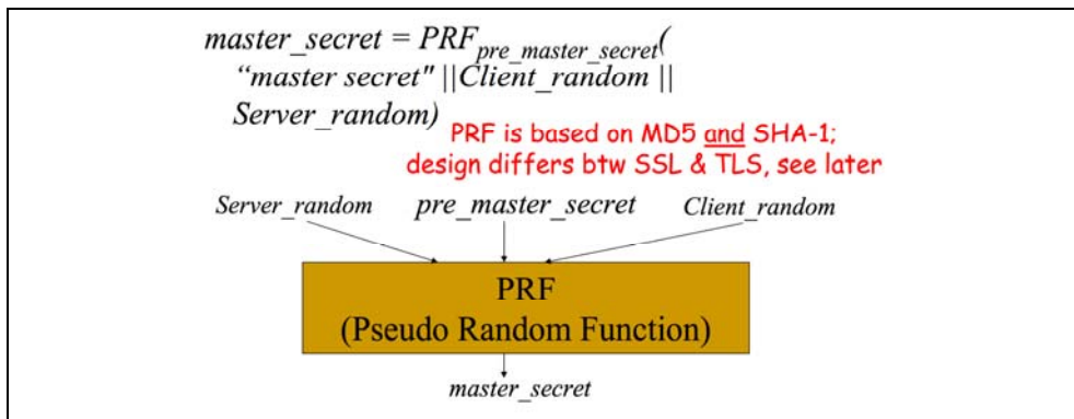
Figure 12-4. Master secret generation
